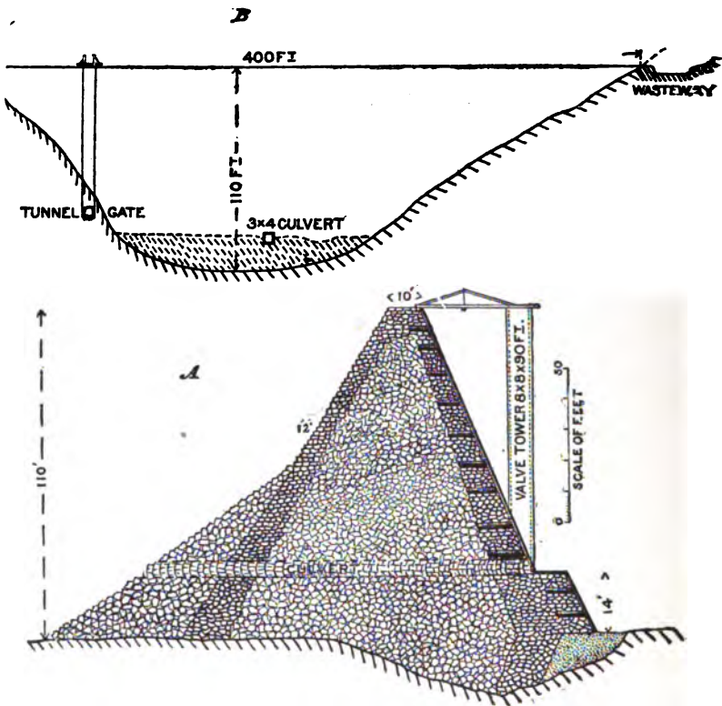
FIG. 215.—Elevation and Cross-section of Walnut Grove Dam.
